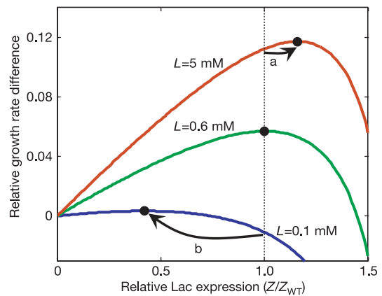
Figure 3 | 3 Predicted relative growth rate of cells (the fitness function) as a function of Lac protein expression. The fitness function, given by the difference of cost and benefit, is shown for different concentrations of lactose. The x axis is the ratio of protein level to the fully induced wild-type protein level, Z/Z_{WT} . Shown are relative growth rate differences with respect to the uninduced wild-type strain for environments with lactose levels L = 0.1 mM (blue line), L = 0.6 mM (green line) and L = 5 mM (red line), according to equation (5). The dot on each line is the predicted optimal expression level that provides maximal growth (equation (6)). Cells grown in lactose levels above 0.6 mM are predicted to evolve to increased Lac protein expression (arrow a), whereas cells grown at lactose levels lower than 0.6 mM are predicted to evolve to decreased Lac protein expression (arrow b).
